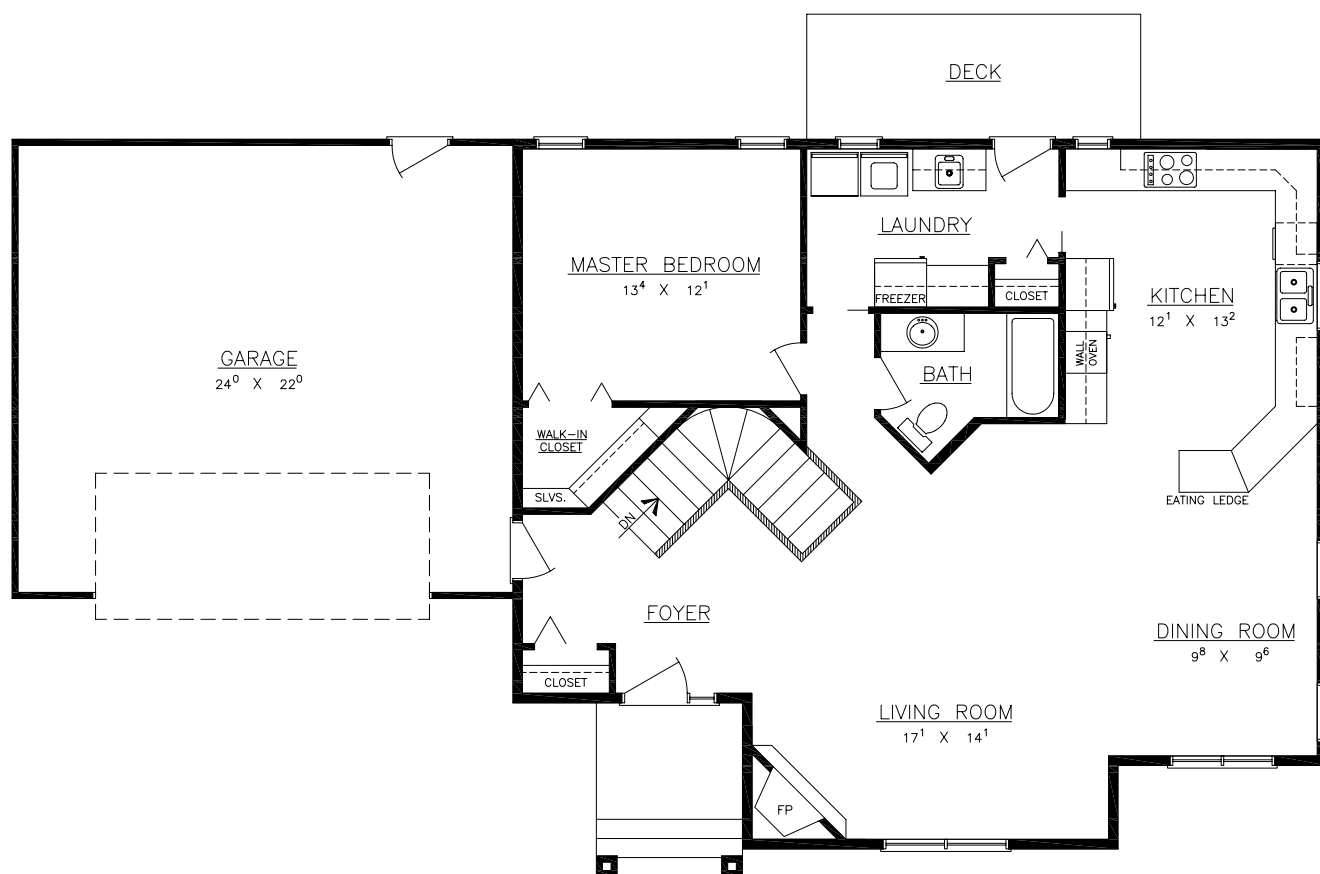
FLOOR PLAN
